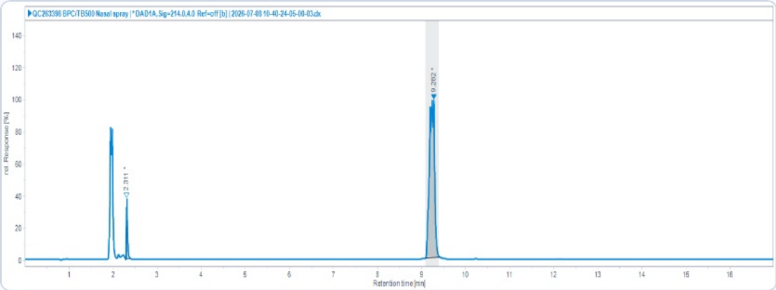
HPLC Chromatogram (Retention Time: 2.311, 9.282 min)
