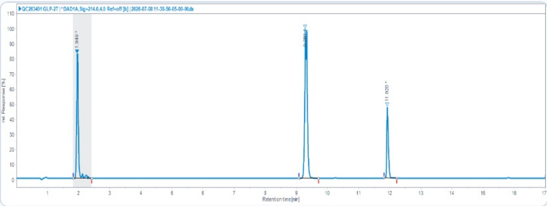
HPLC Chromatogram (Retention Time: 9.281, 11.920 min)
