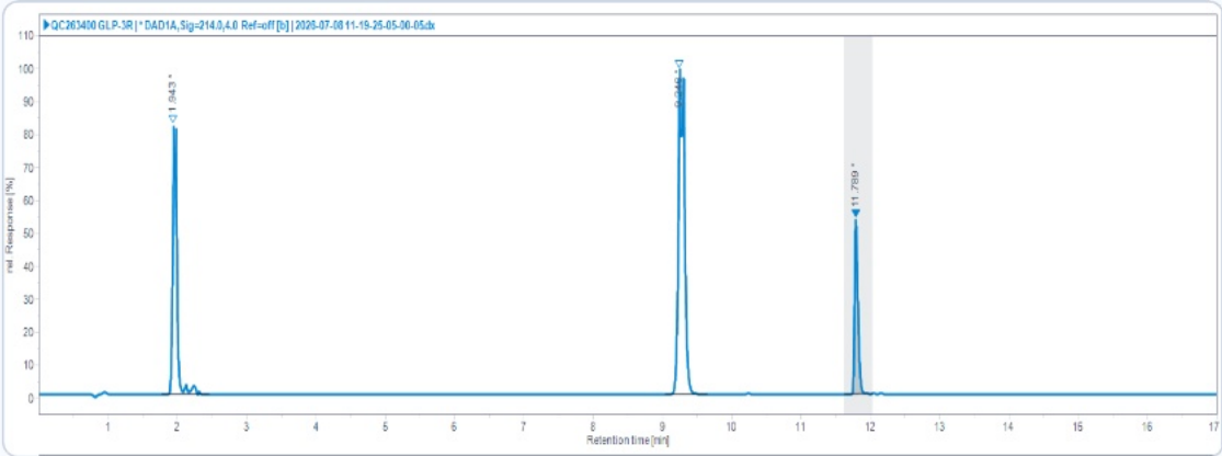
HPLC Chromatogram (Retention Time: 9.246, 11.789 min)
