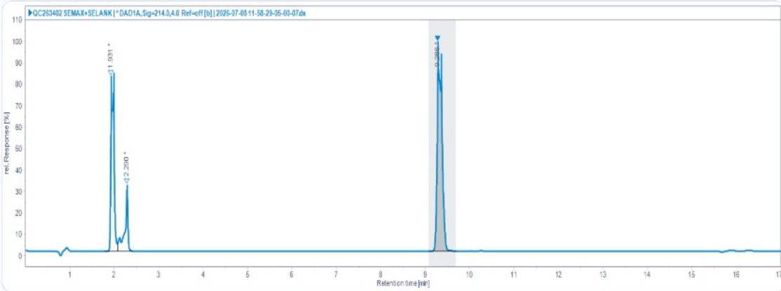
HPLC Chromatogram (Retention Time: 2.290, 9.286 min)
